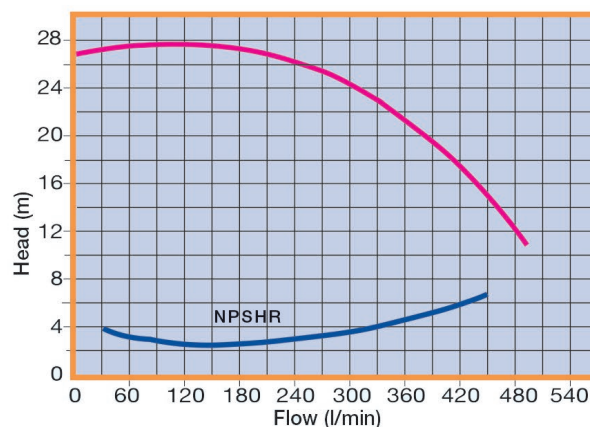
Performance Curve 60 Hz - Rpm 3400
