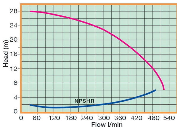
Performance Curve 50 Hz - Rpm 2800
