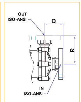
CONNECTION TYPE F
