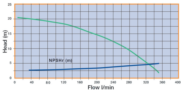
Performance Curve 60 Hz - Rpm 3400
