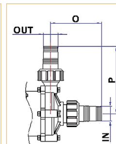
CONNECTION TYPE P
