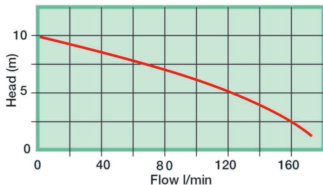
Performance Curve 50 Hz - Rpm 2800
